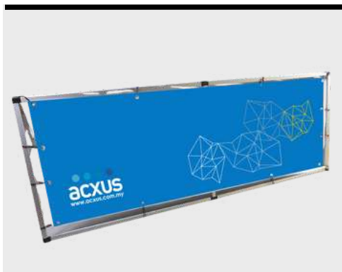
JETA A-V VERTICAL A-BOARD 2625mm x 1110mm PRINTING : 2400mm x 900mm 4.35KG
